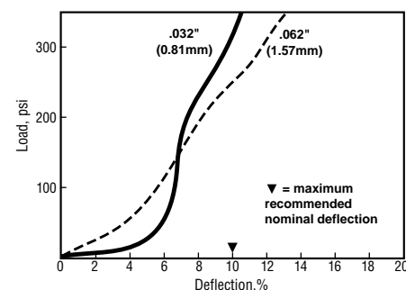
Figure 2 CHO-SEAL 1217 Sheet Stock Compression-Deflection
