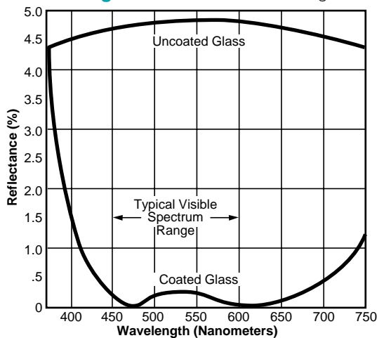
Figure 4 Antireflection Coating
