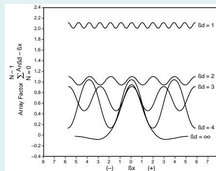
Figure 23 Array Factor vs. Spacing
