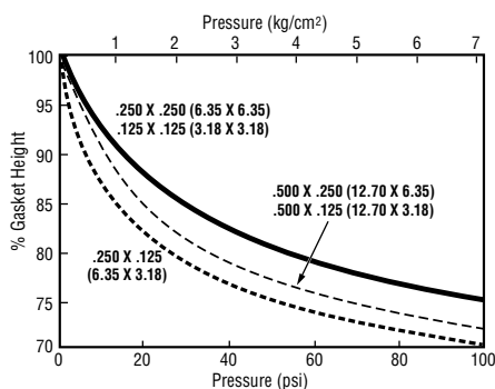
Figure 1 Compression vs. Pressure for MESH STRIP Gasketing
