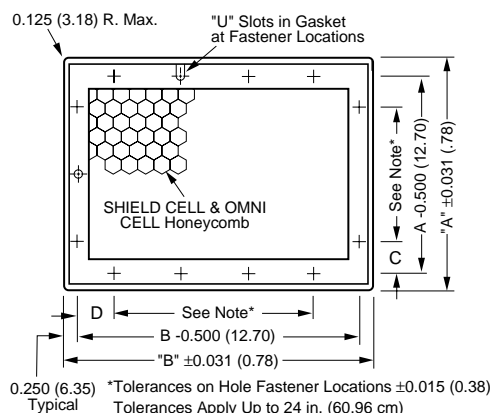
Figure 2 Dimensions for SHIELD CELL and OMNI CELL Vent Panels
