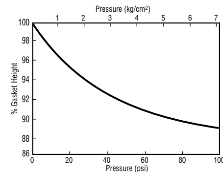
Figure 7 Compression vs. Pressure for PORCUPINE METALASTIC Gasketing
