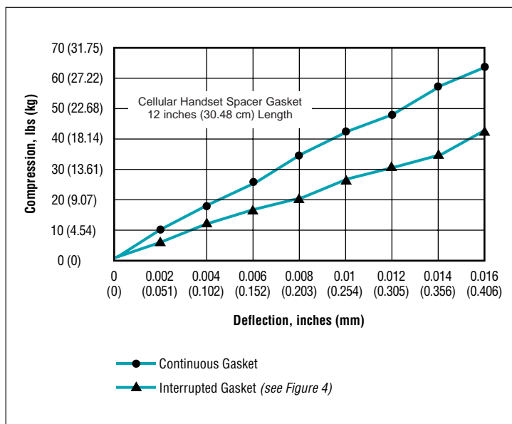
Figure 5 Typical Spacer Gasket Deflection
