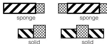
Figure 37 Normal and High Pressure COMBO STRIP Gaskets
