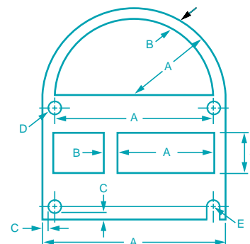
Figure 1 Dimensions for METALASTIC and PORCUPINE METALASTIC Die-Cut Gaskets
