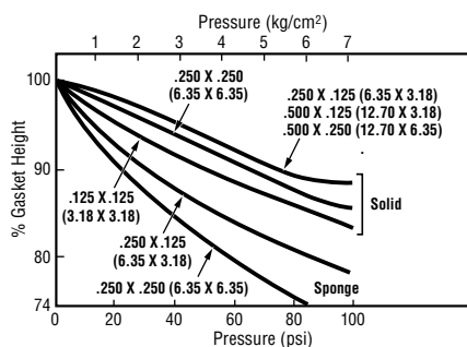
Figure 5 Compression vs. Pressure for POLASTRIP Gasketing
