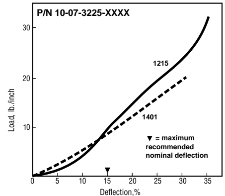
Figure 16 0.125 in. (3.18 mm) Wide Rectangular Strip Compression-Deflection
