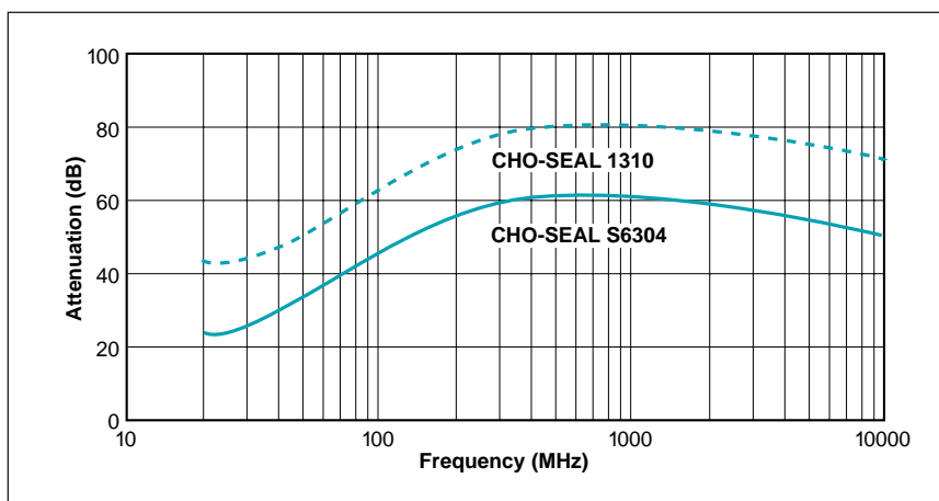
Figure 1 Shielding Effectiveness
