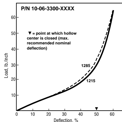
Figure 23 0.250 in. (6.35 mm) Dia. Hollow P-Strip Compression-Deflection
