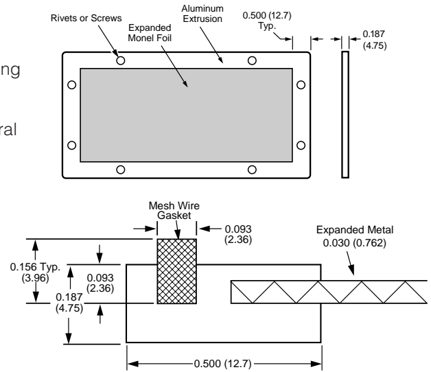
Frame Design 61-448
