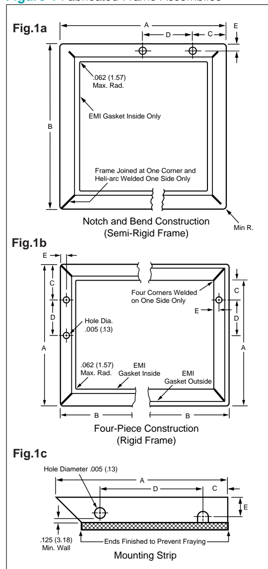
Figure 1 Fabricated Frame Assemblies
