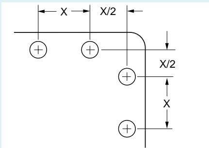
Figure 19 Fastener Location Near Corners
