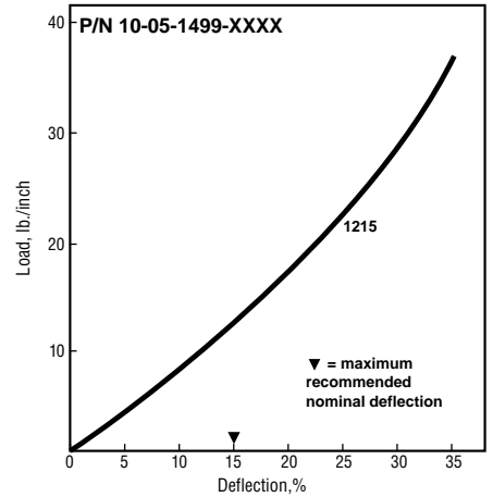
Figure 14 0.156 in. (3.96 mm) High D-Strip Compression-Deflection
