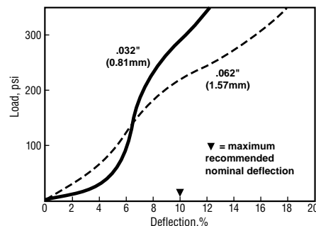
Figure 1 CHO-SEAL 1215 Sheet Stock Compression-Deflection
