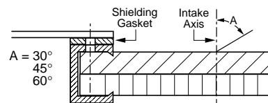
Figure 4 OMNI CELL Drip-Proof Construction
