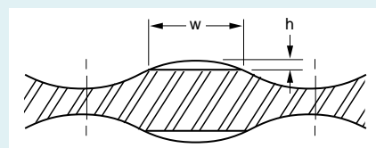
Figure 27 Unfilled Slot is Free to Radiate When Spacing is Equal to 1/2 Wavelength
