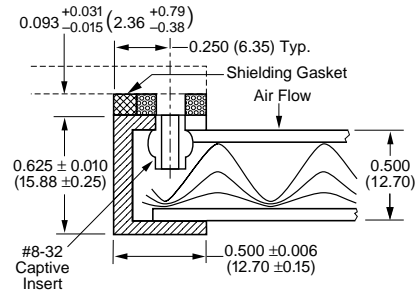
Figure 1 Standard Frame Design 61-118
