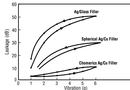
Figure 33 Effects of Vibration on Shielding Effectiveness of Conductive Elastomer Gaskets
