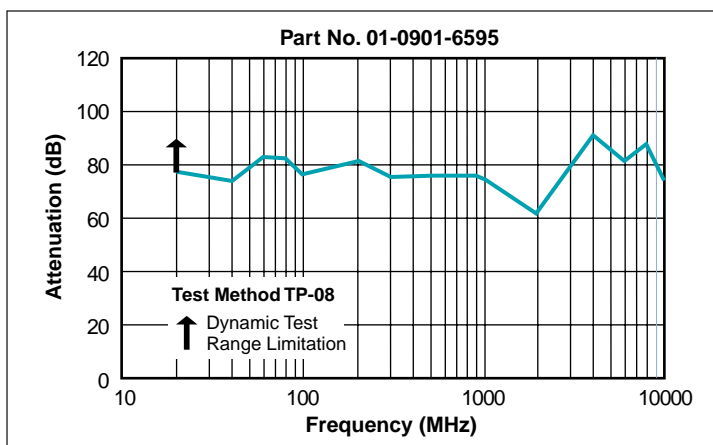
Figure 2 Shielding Effectiveness
