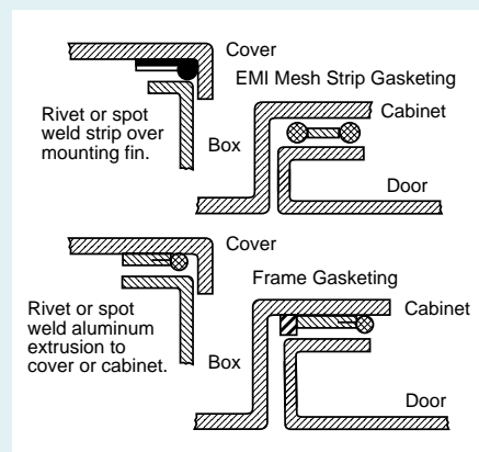
Figure 33 Rivet or Spot Welding
