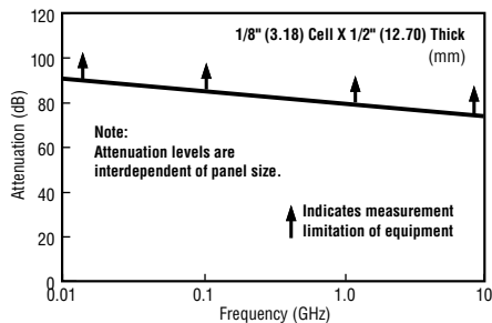
Figure 2 Shielding Effectiveness of CHO-CELL Vents
