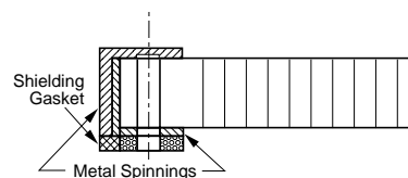
Figure 4 OMNI CELL Drip-Proof Construction
