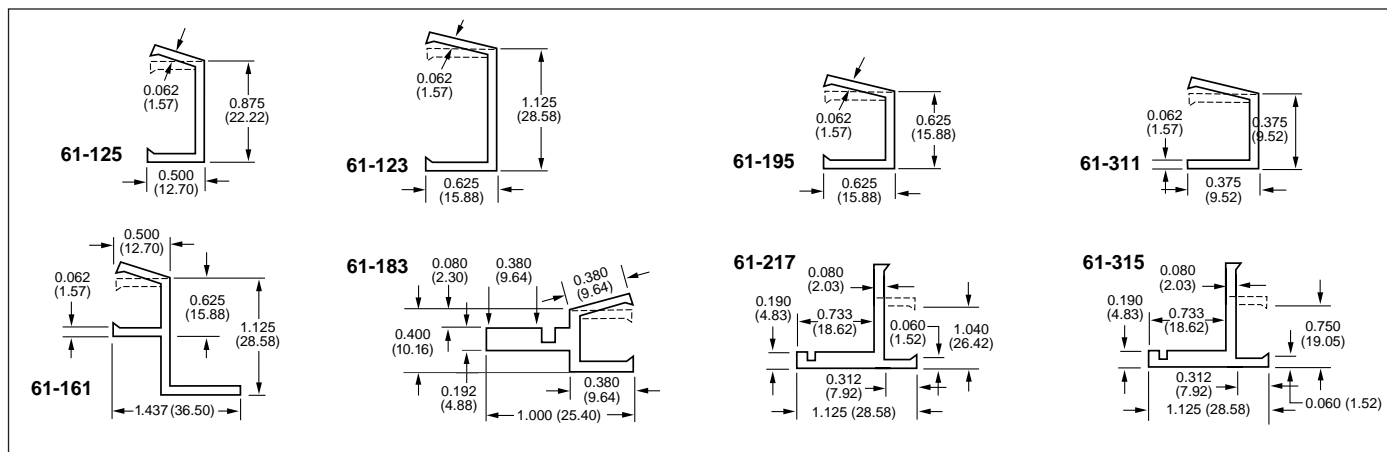
Figure 2 Alternate Extrusions for CHO-CELL Construction, in. (mm). Others available, please inquire.
