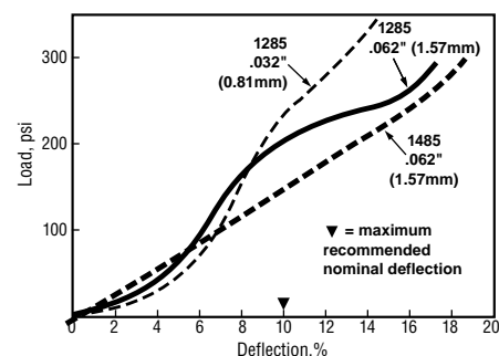
Figure 3 CHO-SEAL 1285 and CHO-SIL 1485 Sheet Stock Compression-Deflection
