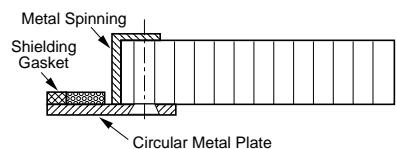
Figure 5 Circular panels
