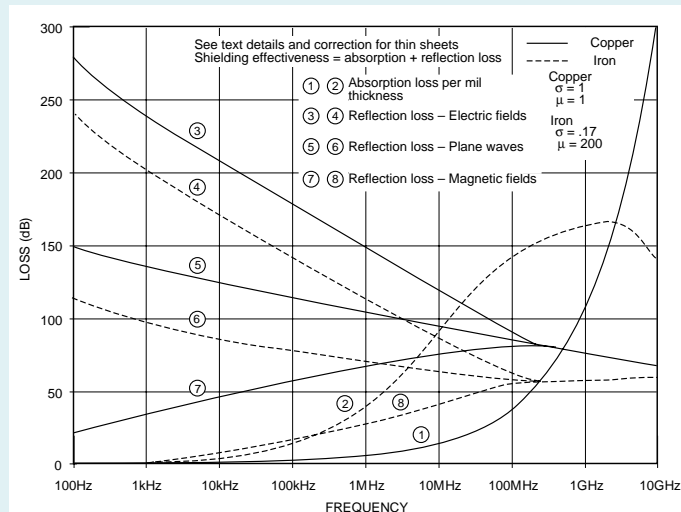
Figure 5 Shielding Effectiveness of Metal Barriers
