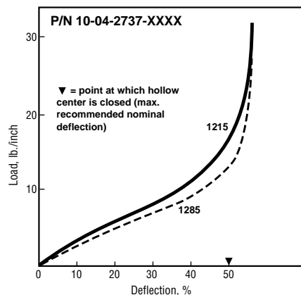
Figure 20 0.250 in. (6.35 mm) Dia. Hollow O-Strip Compression-Deflection
