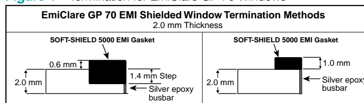
Figure 1 – Termination for EmiClare GP 70 Windows
