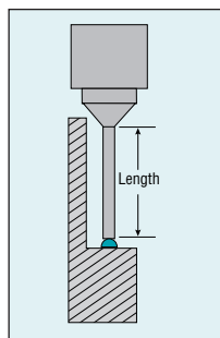
Figure 9 High sidewalls may necessitate longer needles, reducing speed
