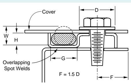
Figure 11a Shaped Sheet Metal Container
