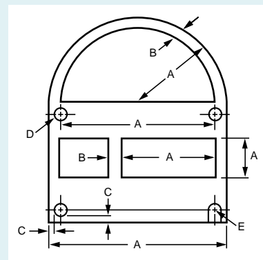
Figure 40 PORCUPINE METALASTIC Die-Cut Gaskets (fully dimensioned drawings required)
