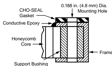
Cross Section of CHO-CELL Vent
