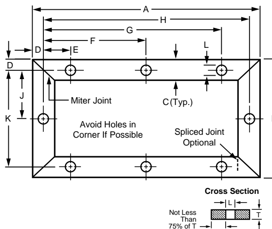
Figure 2 Dimensions and Tolerances for POLASTRIP and COMBOPOLASTRIP Fabricated Gaskets
