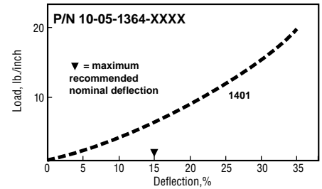
Figure 13 0.135 in. (3.43 mm) High D-Strip Compression-Deflection
