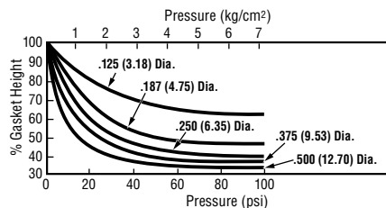
Figure 3 Compression vs. Pressure for Monel Round MESH STRIP Gasketing
