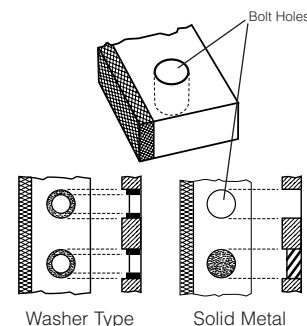
Figure 1 Compression Stops
