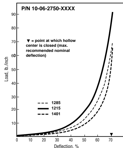
Figure 24 0.360 in. (9.14 mm) Dia. Hollow P-Strip Compression-Deflection
