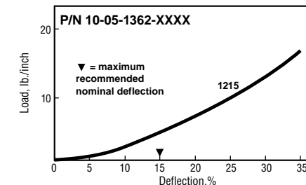
Figure 12 0.068 in. (1.73 mm) High D-Strip Compression-Deflection
