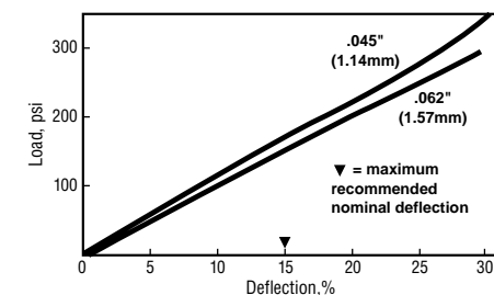
Figure 4 CHO-SIL 1401 Sheet Stock Compression-Deflection
