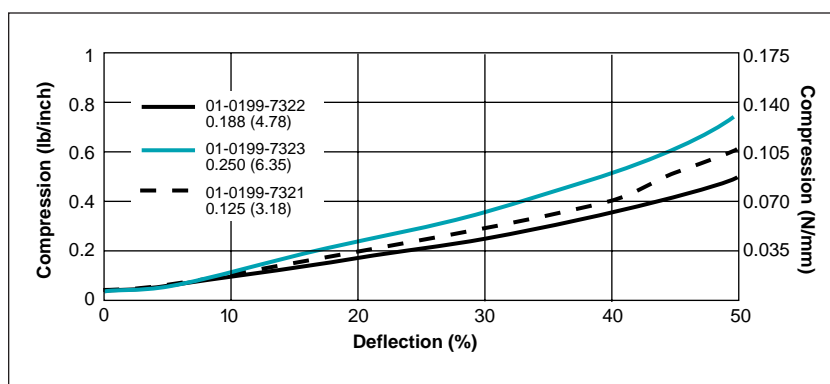
Figure 2 Compression-Deflection
