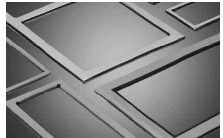
Individually 360° wrapped picture-frame and ladder gaskets available in SOFT-SHIELD 4000, 4006 and 4008 materials.
