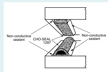
Figure 16 “Seal-to-seal” design incorporating CHO-SEAL® 1287 conductive silver-aluminum fluorosilicone gaskets on both mating flange surfaces. Gaskets are bonded and edge sealed to prevent moisture from entering the gasket/flange area.
