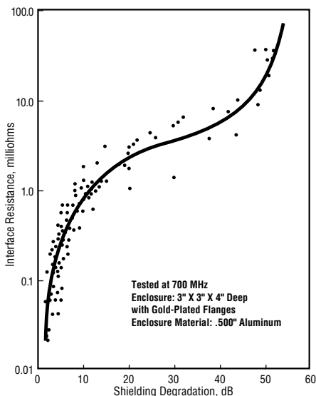
Figure 30 Interface Resistance vs. Shielding Degradation at a Flange Joint
