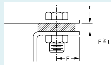
Figure 12 Flat Gasket on Sheet Metal Flange
