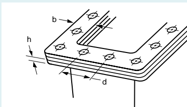
Figure 22 Bolt Spacings for Flanges
