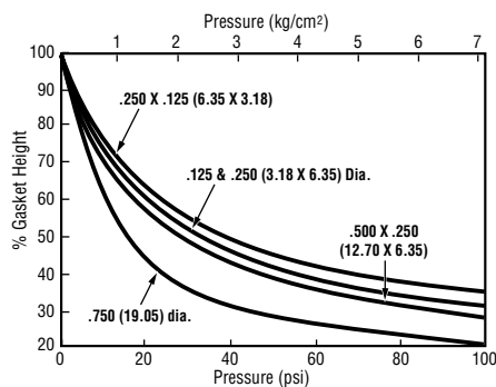
Figure 4 Compression vs. Pressure for MESH STRIP Gasketing with Neoprene Sponge Core and Two Layers of Monel Mesh
