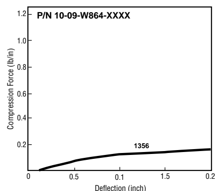
Figure 25 0.410 in. (10.41 mm) High V-Strip Compression-Deflection
