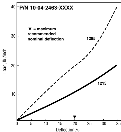
Figure 8 0.125 in. (3.18 mm) Dia. O-Strip Compression-Deflection
