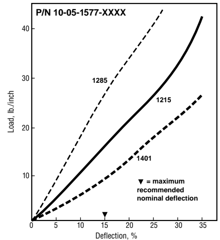
Figure 15 0.175 in. (4.45 mm) High D-Strip Compression-Deflection
