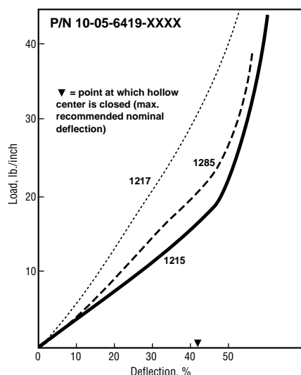
Figure 21 0.156 in. (3.96 mm) High Hollow D-Strip Compression-Deflection
