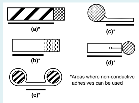
Figure 31 a-d Application of Non-Conductive Adhesive
