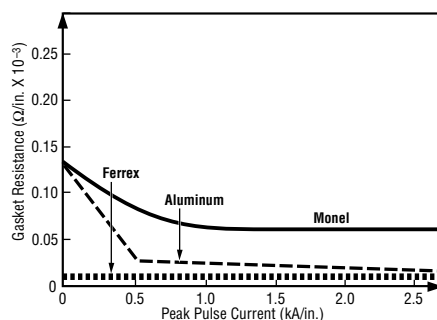
Figure 13 EMP Current Response of Mesh Gaskets
