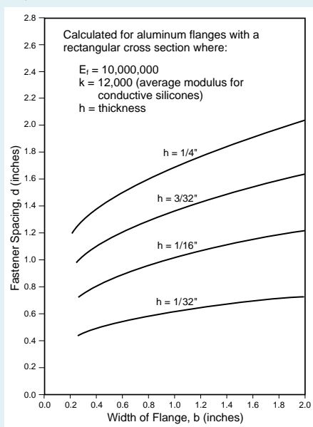
Figure 24 Fastener Spacing
