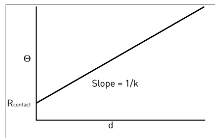
Figure 2. Thermal Impedance vs. Thickness
