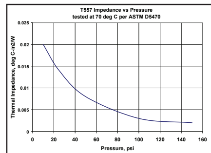
Figure 1b. Interface material compressed between two contacting surfaces
